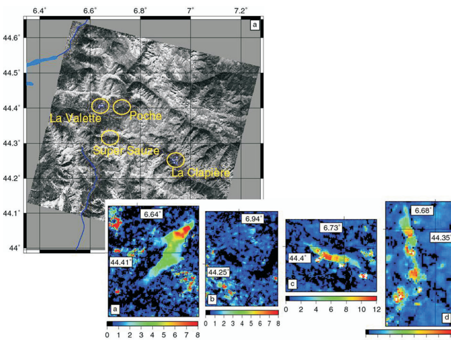
FIG. 5. – Horizontal displacement maps (m) over the French South Alps derived from the correlation of SPOT5 images (2003, 09/19 – 2004, 08/22). Three major landslides are clearly visible: a) “La Valette” mudslide, c) “Poche” mudslide and d) “Super Sauze” mudslide; b) “La Clapière” landslide is more difficult to discriminate.
