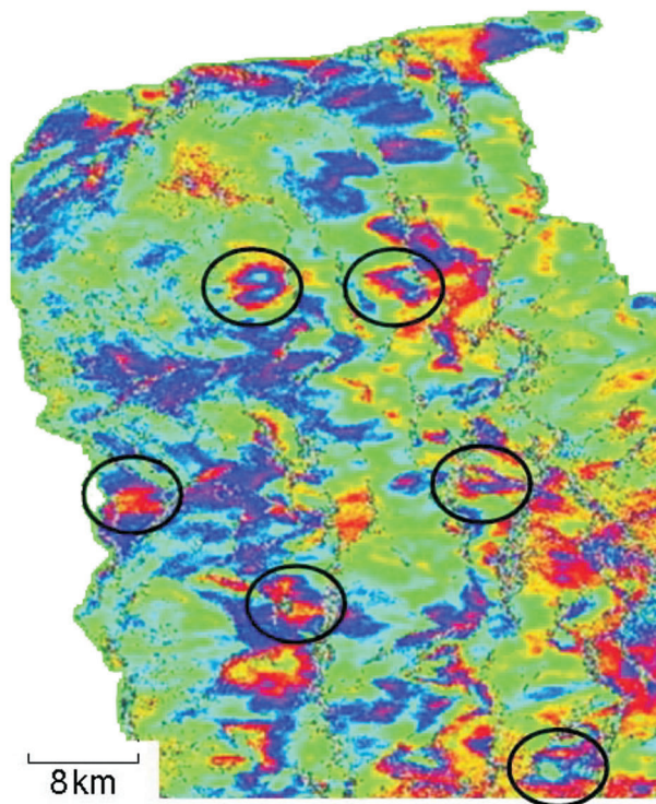
FIG. 3 – Example of bias (black dots) due to tropospheric heterogeneities occurring within 1 day (1995, October 22-23) differential interferogram over the French South Alps.
